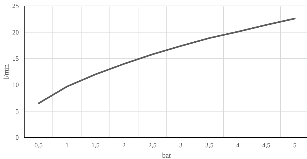
QS3300 - built-in part only (flowrate L/min)
