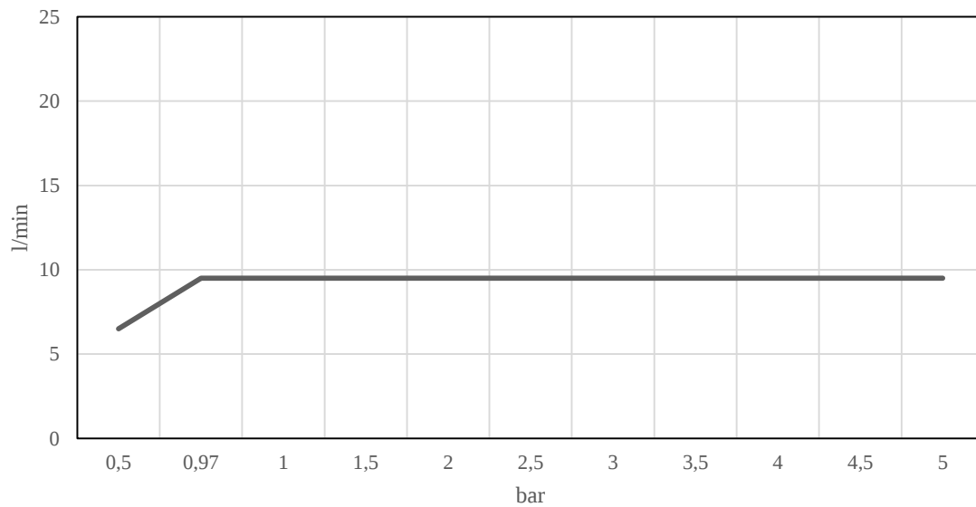
QS3300-340Sxxx (flowrate L/min)
